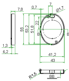
Cover
