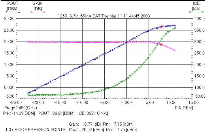
Figure 2 – Power Sweep (Vc = 3.3V, Vref = 2.85V, Icq = 65mA)
