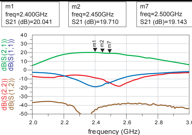
Figure 6 – S-Parameter Data (Vc = 4.5V, Vref = 2.85V, Icq = 65mA)
